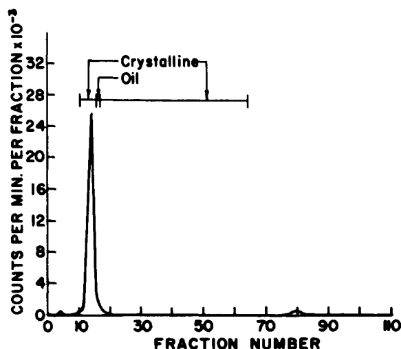
FIG. 2.—Radiochromatogram of material which was extractable into ether after saponification. The material was obtained from 5.5 g of seeds grown for 5 days in the presence of 266,000 cpm of d,l -2- C^{14} -mevalonic acid. Radioactivity in the peak near fraction 14 was derived from \beta -amyrin, as shown by further isolation. The crystalline material following the \beta -amyrin was \beta -sitosterol. The details of the solvents used for elution are given in Figure 3, which represents the same chromatogram on an expanded scale for the ordinate.
