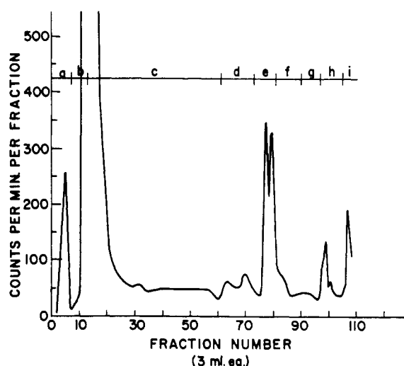
FIG. 3.—Radiochromatogram of material which was extractable into ether after saponification. The material was obtained from 5.5 g of seeds grown for 5 days in the presence of 266,000 cpm of d,l -2- C^{14} -mevalonic acid. In the chromatogram the following elutions were made: (a) 30% ether in light petroleum ether; (b) 40% ether in petroleum ether; (c) 50% ether in petroleum ether; (d) ether; (e) 1% ethanol in ether; (f) 2% ethanol in ether; (g) 5% ethanol in ether; (h) 10% ethanol in ether; and (i) 25% ethanol in ether.
